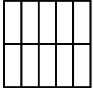
Color \frac{5}{10}
