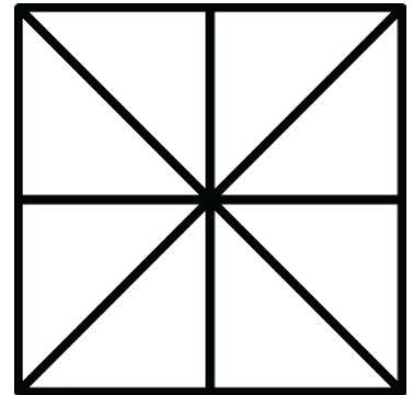
Color \frac{4}{8}
