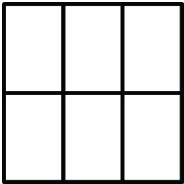
Color \frac{2}{6}
