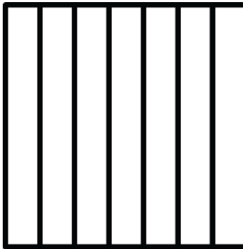
Color \frac{4}{7}
