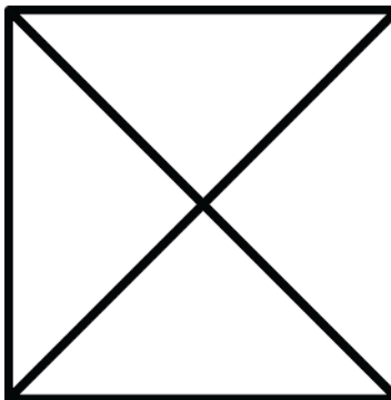
Color \frac{2}{4}
