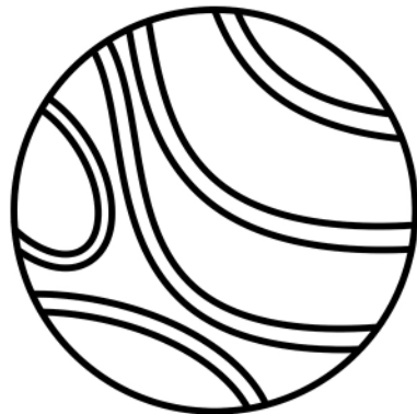
NEPTUNE
