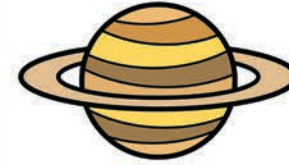
Saturn
