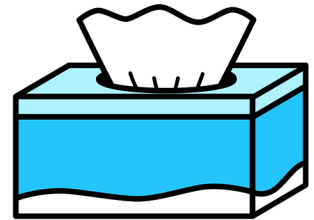
cuboid
