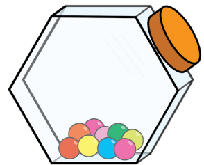
hexagonal prism
