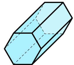
hexagonal prism
